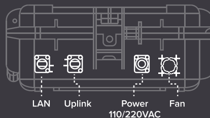
RIGHT VIEW
